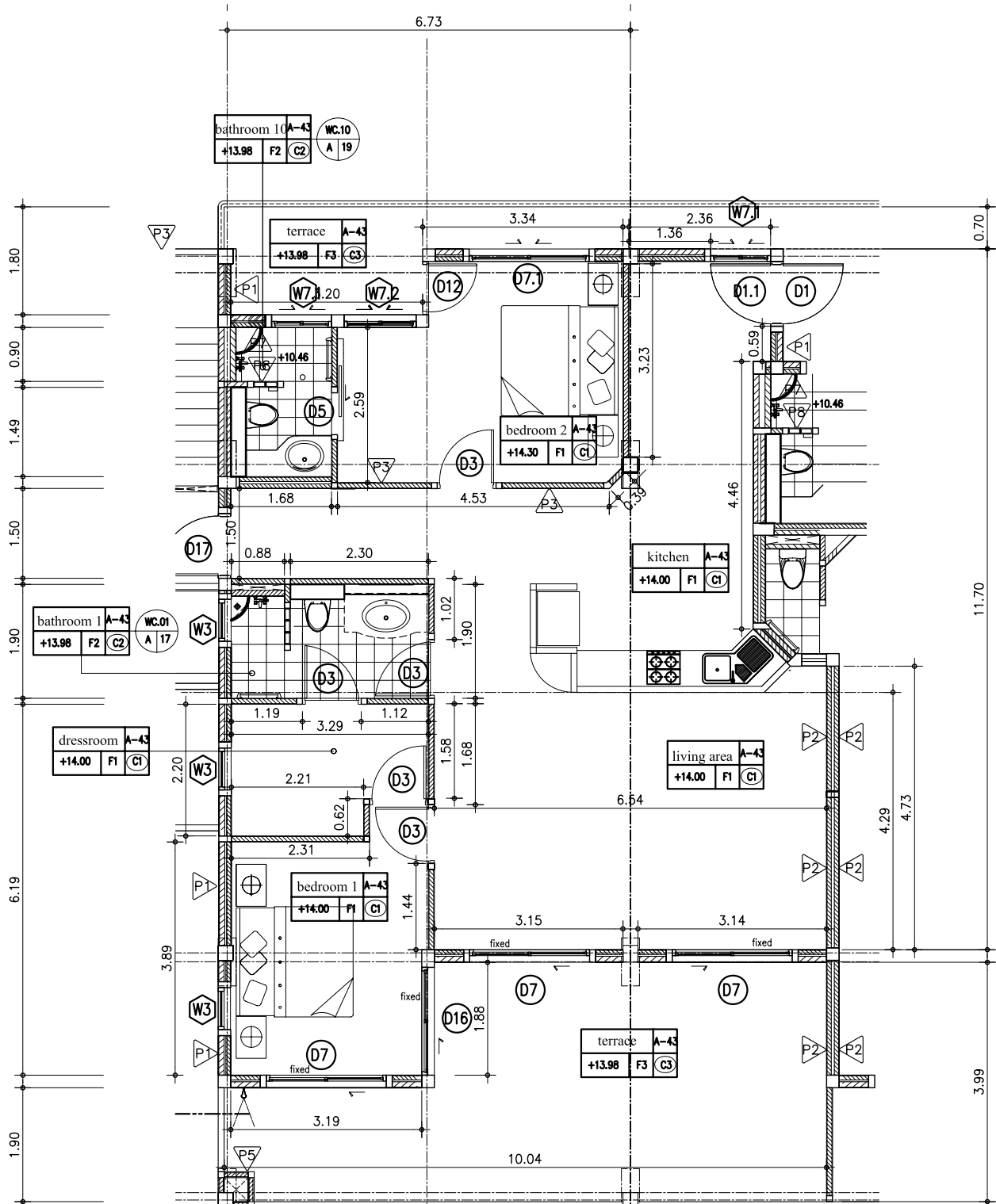
A-43 4 th FLOOR PLAN 1:100 HIGHRISE BUILDING PHASE 1
