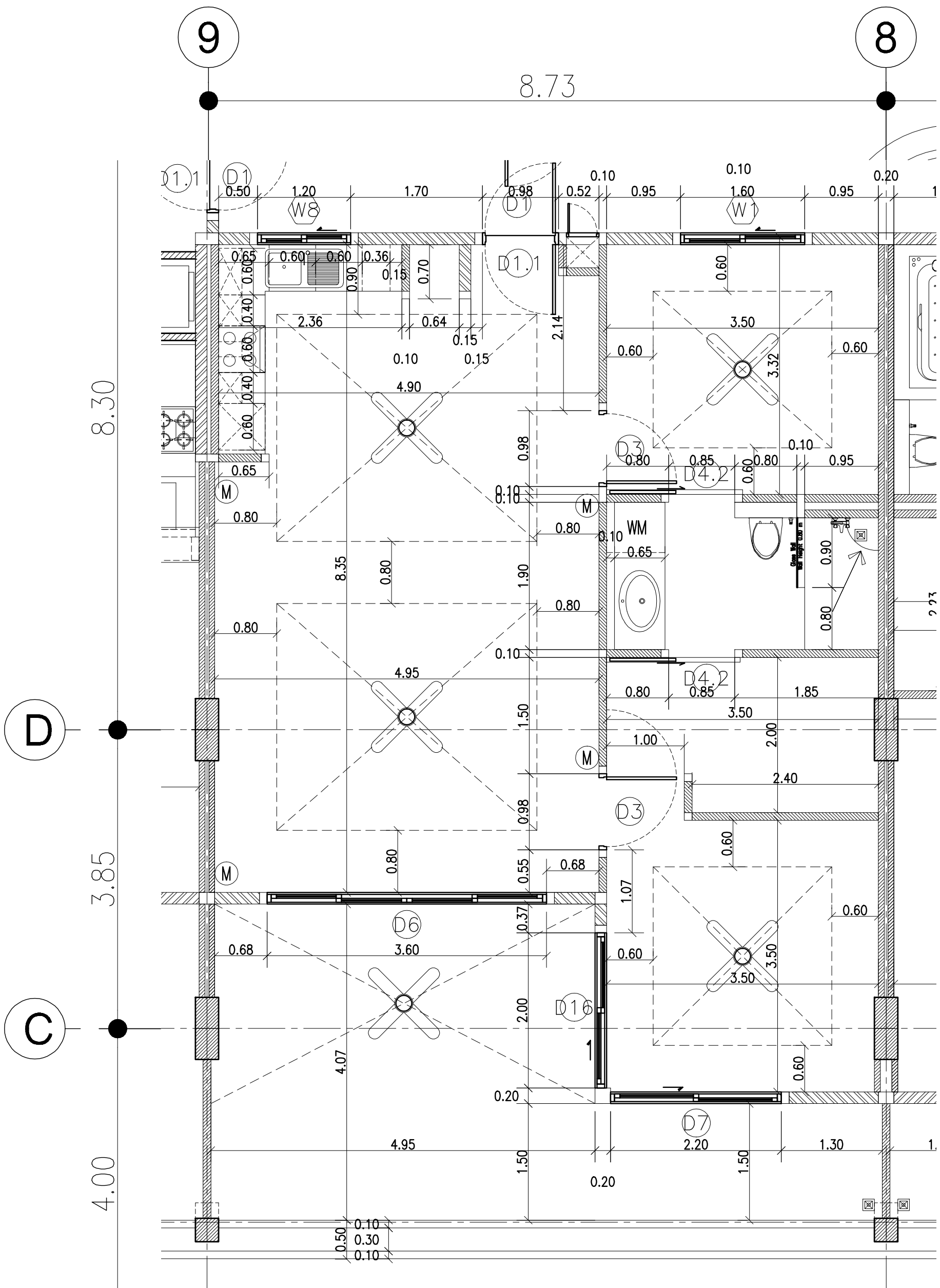
B-32 (3 Floor Plan)
